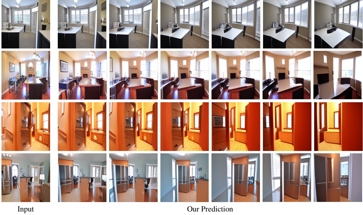
Figure 7. Long-term view synthesis on RealEstate10K [74]. Our method is able to synthesize consistent novel views with large camera transformations while maintaining high fidelity.
