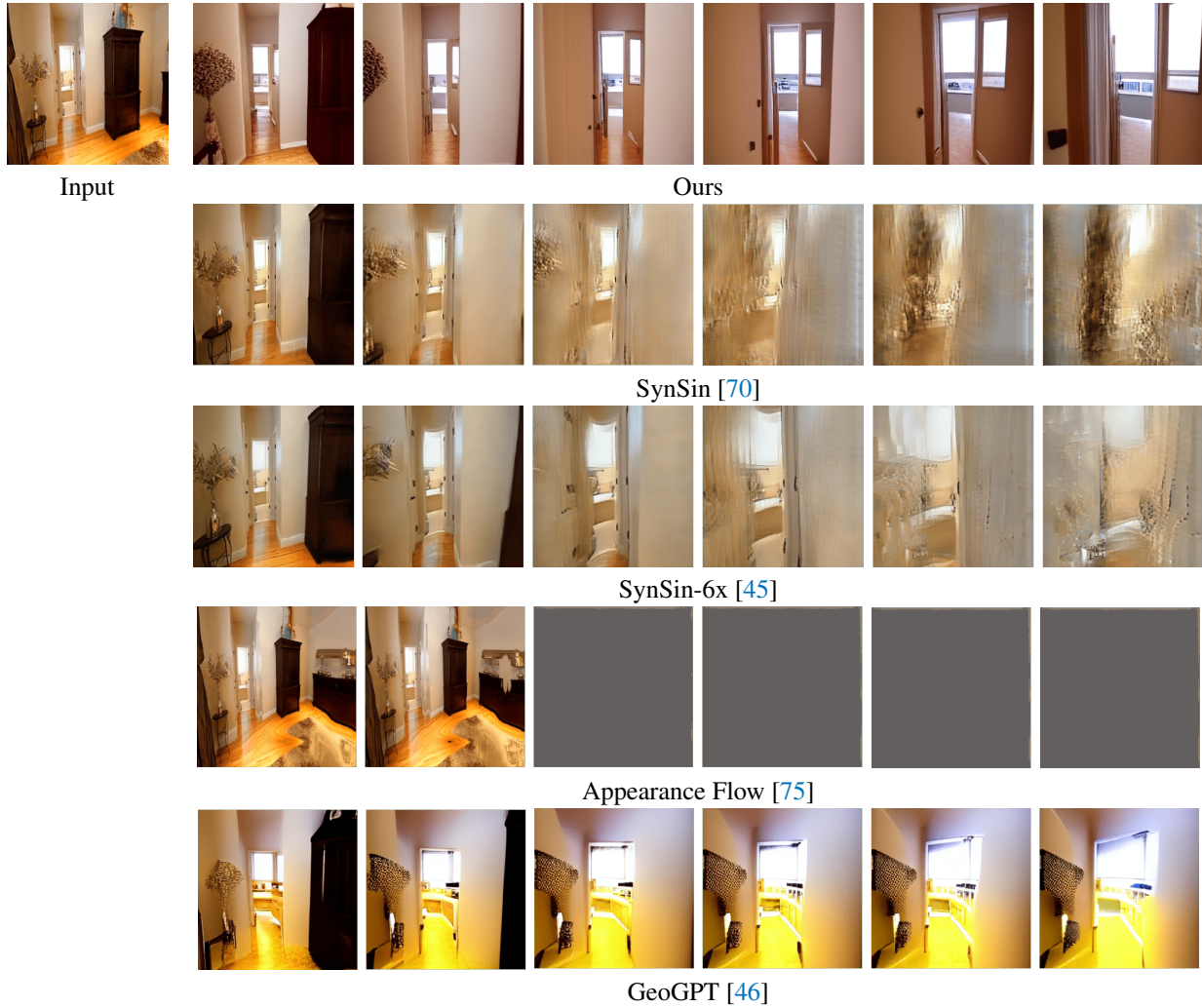
Figure 9. Long-term view synthesis compared with baselines. Previous methods are not capable of synthesizing a consistent long-term scene video. Our method can synthesize long-term views of perceptual consistency and high-fidelity.
